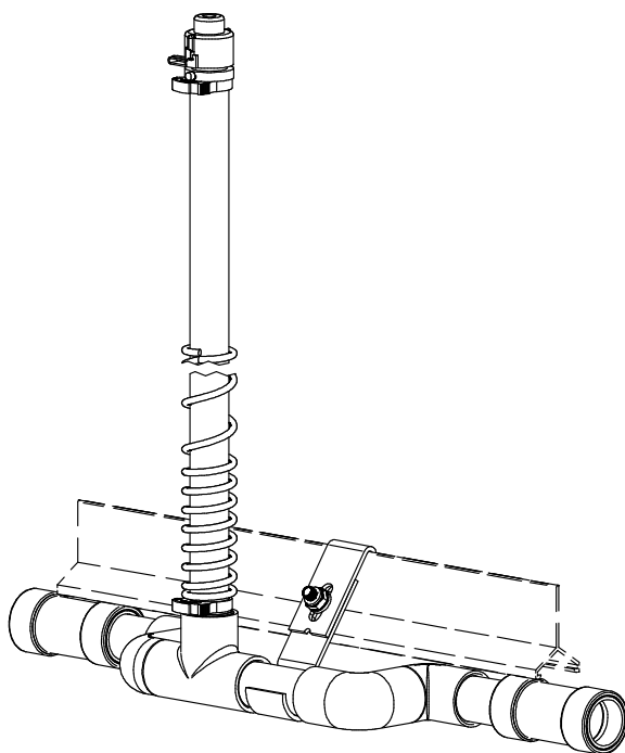
ASSEMBLED VIEW
