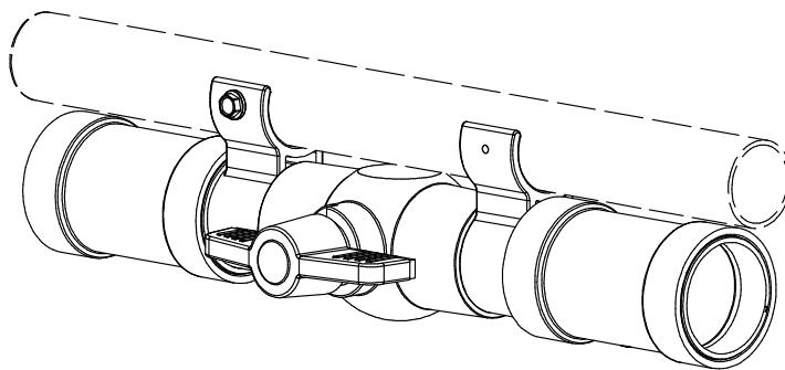
ASSEMBLED VIEW
