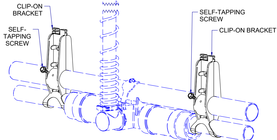
ACE VERSION PN XP-00547 ASSEMBLY: ACE CLIP-ON BRACKET W/SCREWS
