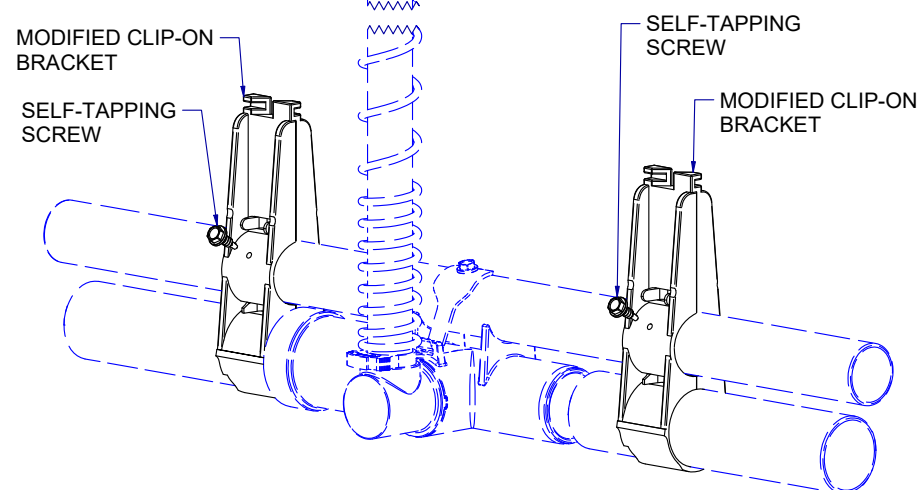
BIG ACE/BIG Z/1" PVC VERSION PN XP-00532 ASSEMBLY: MODIFIED CLIP-ON BRACKET W/SCREWS
